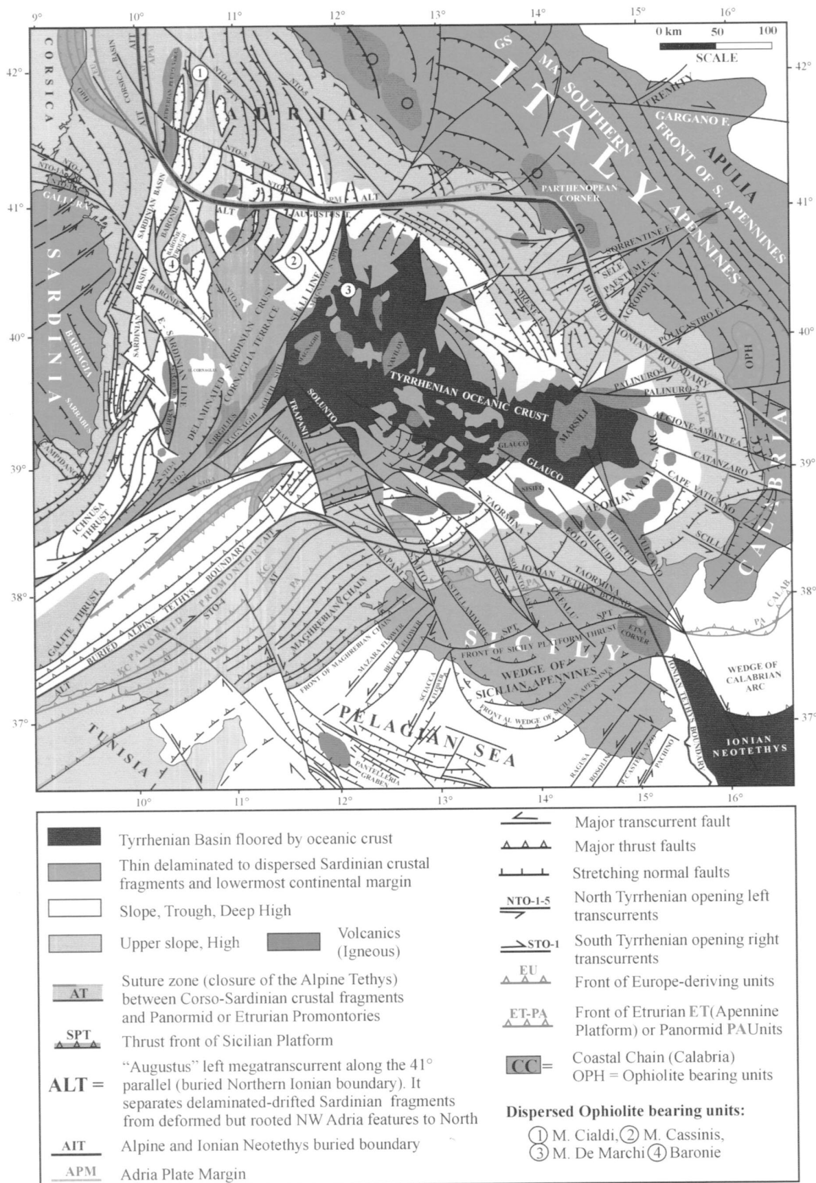
Fig. 9 – Tectonic scheme of the Tyrrhenian Sea and surrounding geological provinces.
